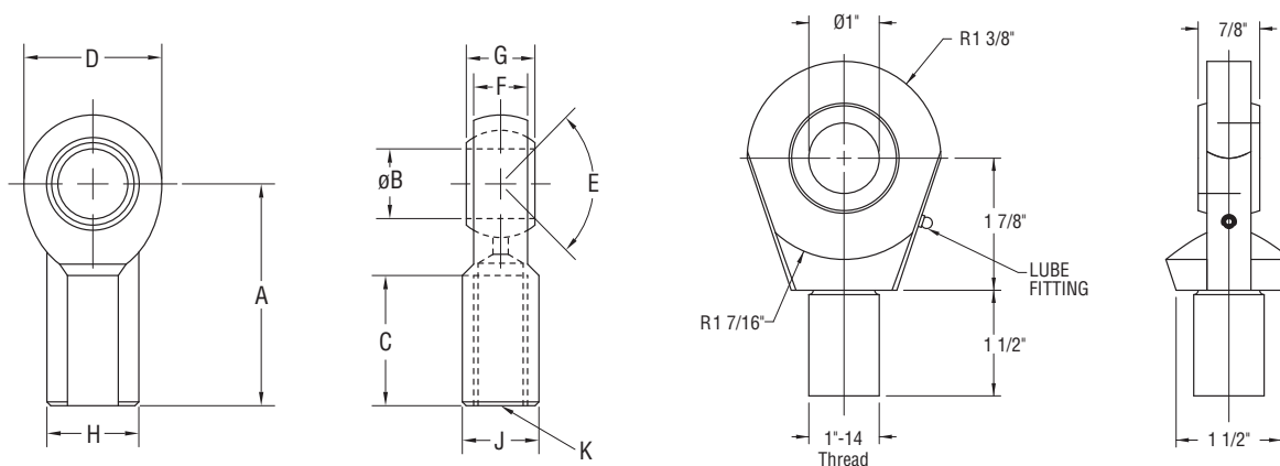
Dimensions for SRM038, SRM044, SRM075
