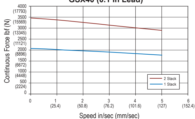
GSX40 (0.1 In Lead)
