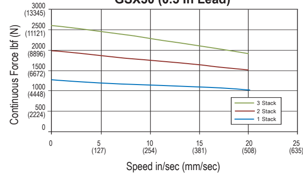
GSX50 (0.5 In Lead)
