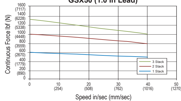
GSX50 (1.0 In Lead)
