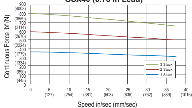
GSX40 (0.75 In Lead)
